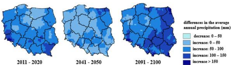
Figure 6. Difference in average annual precipitation (mm) in Poland for the periods 2011-2020, 2041-2050, and 2091-2100 relative to 1971-2000 under the RCP4.5 scenario and simulation of the RACMO22E model.
